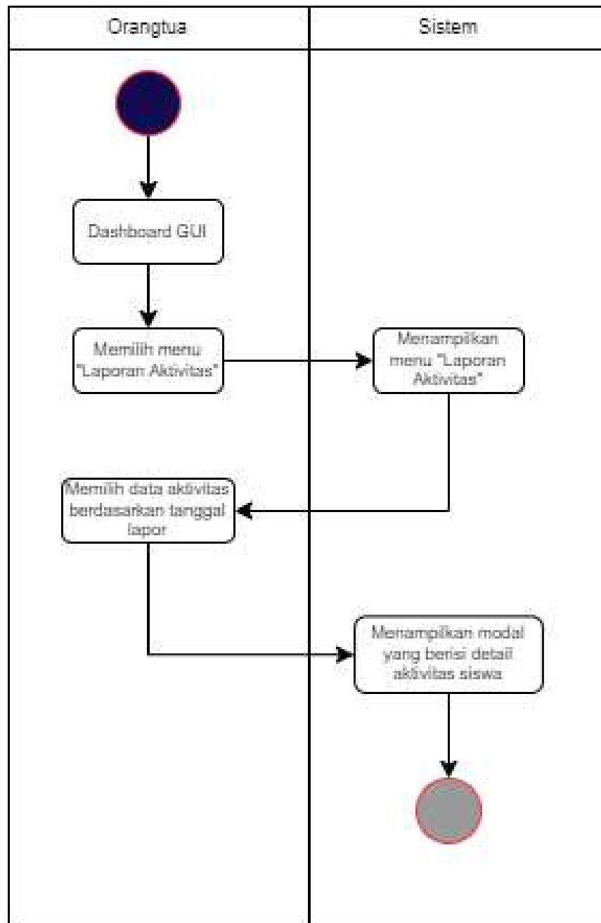
Gambar 3. 7 Activity Diagram View Laporan Aktivitas Siswa
