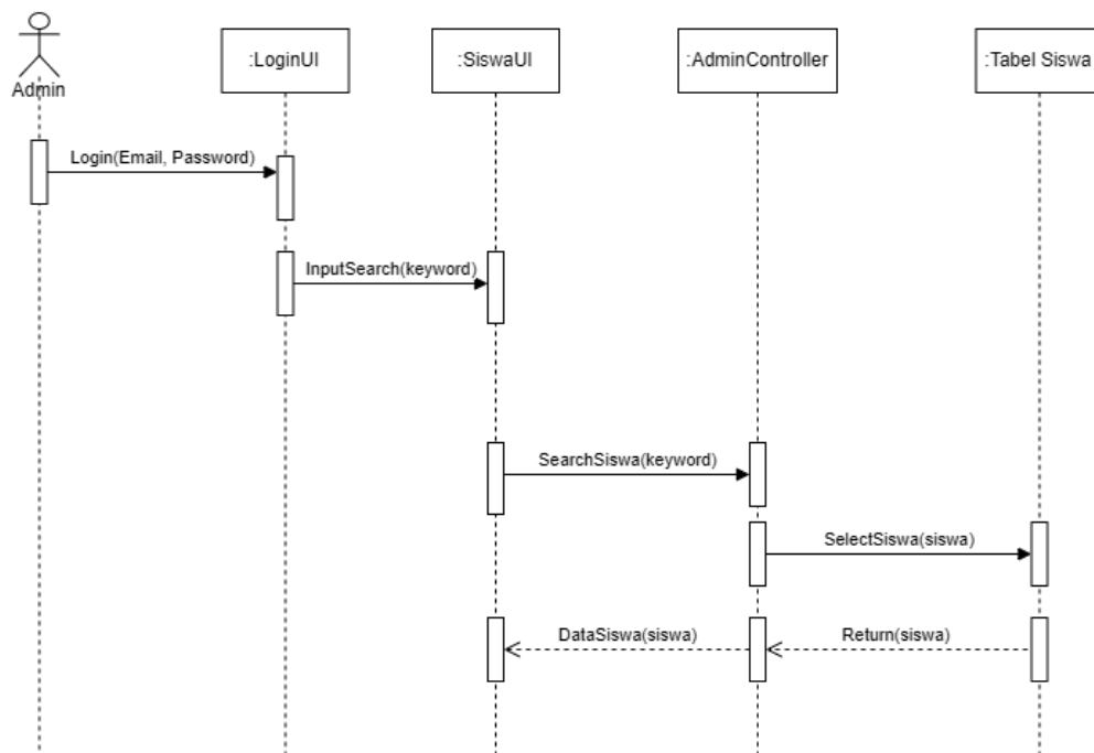
Gambar 3. 18 Sequence Diagram Search Siswa
