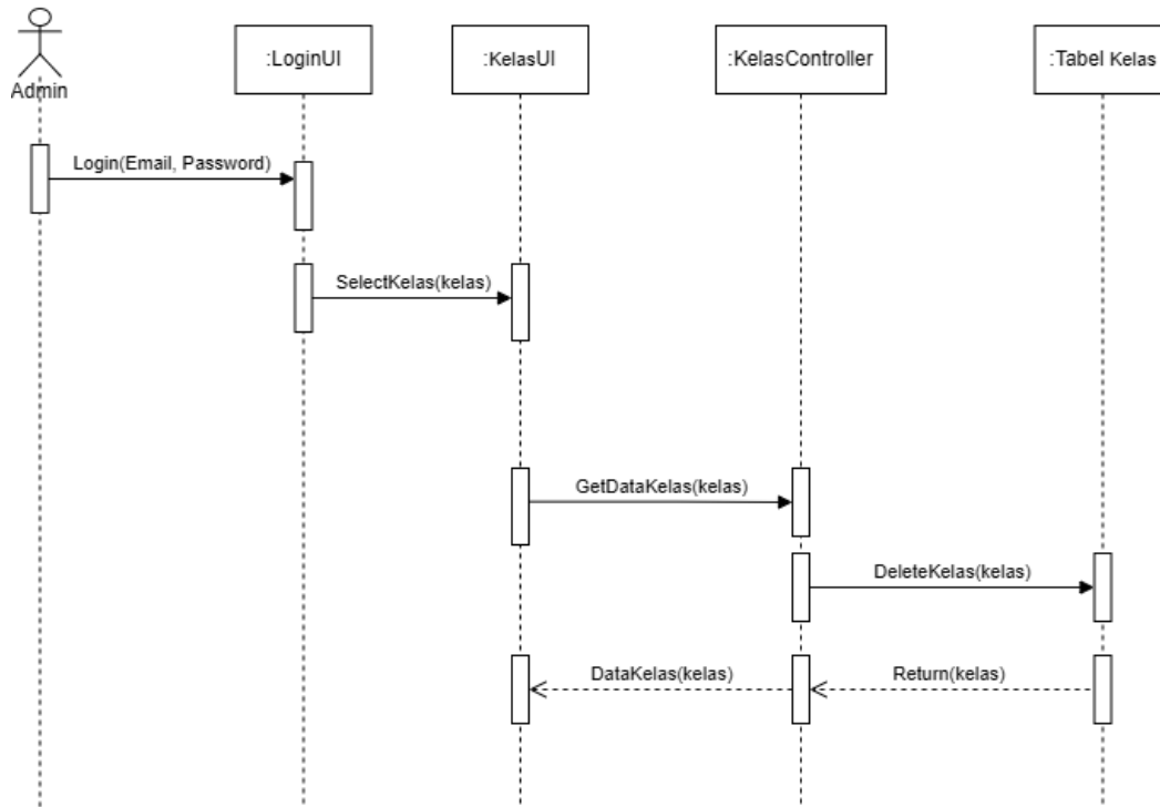
Gambar 3. 31 Sequence Diagram Delete Kelas
