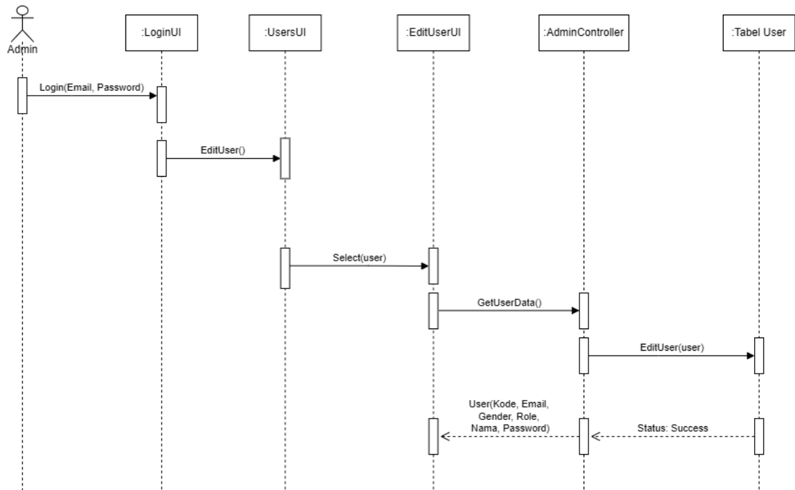
Gambar 3. 11 Sequence Diagram Edit User
