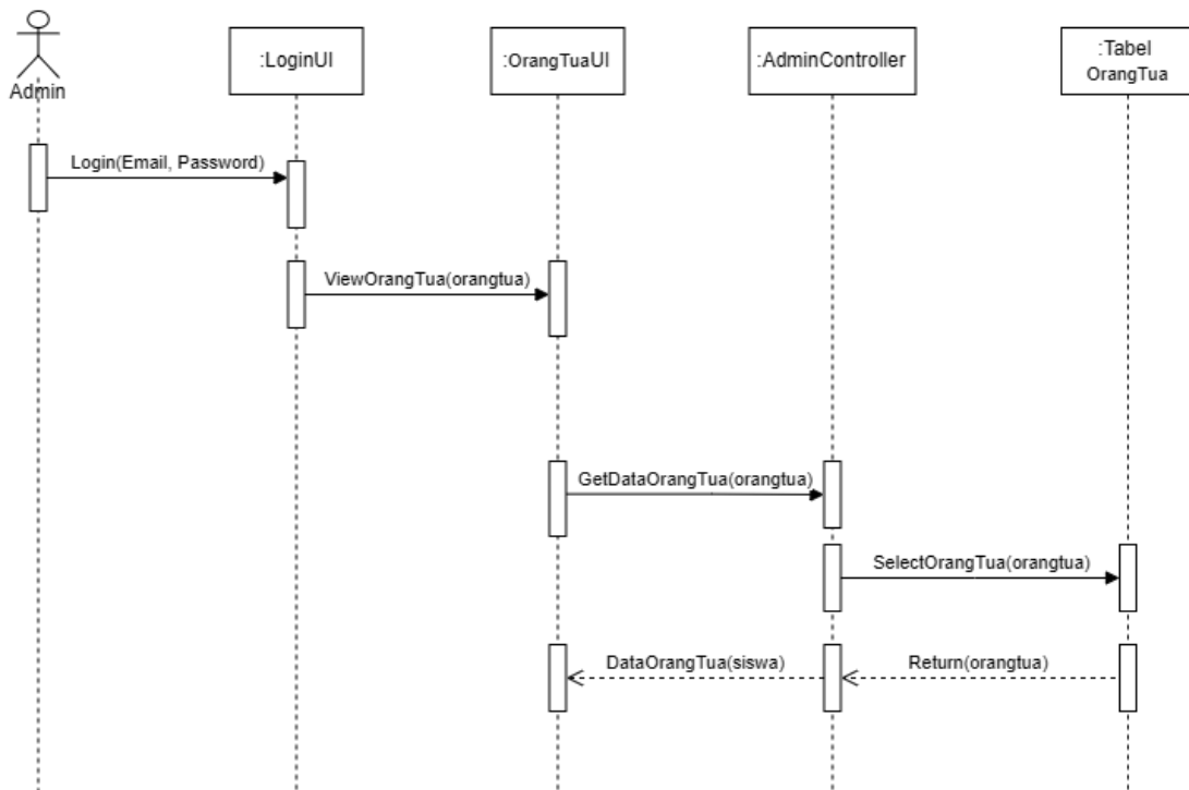
Gambar 3. 23 Sequence Diagram View Orang Tua
