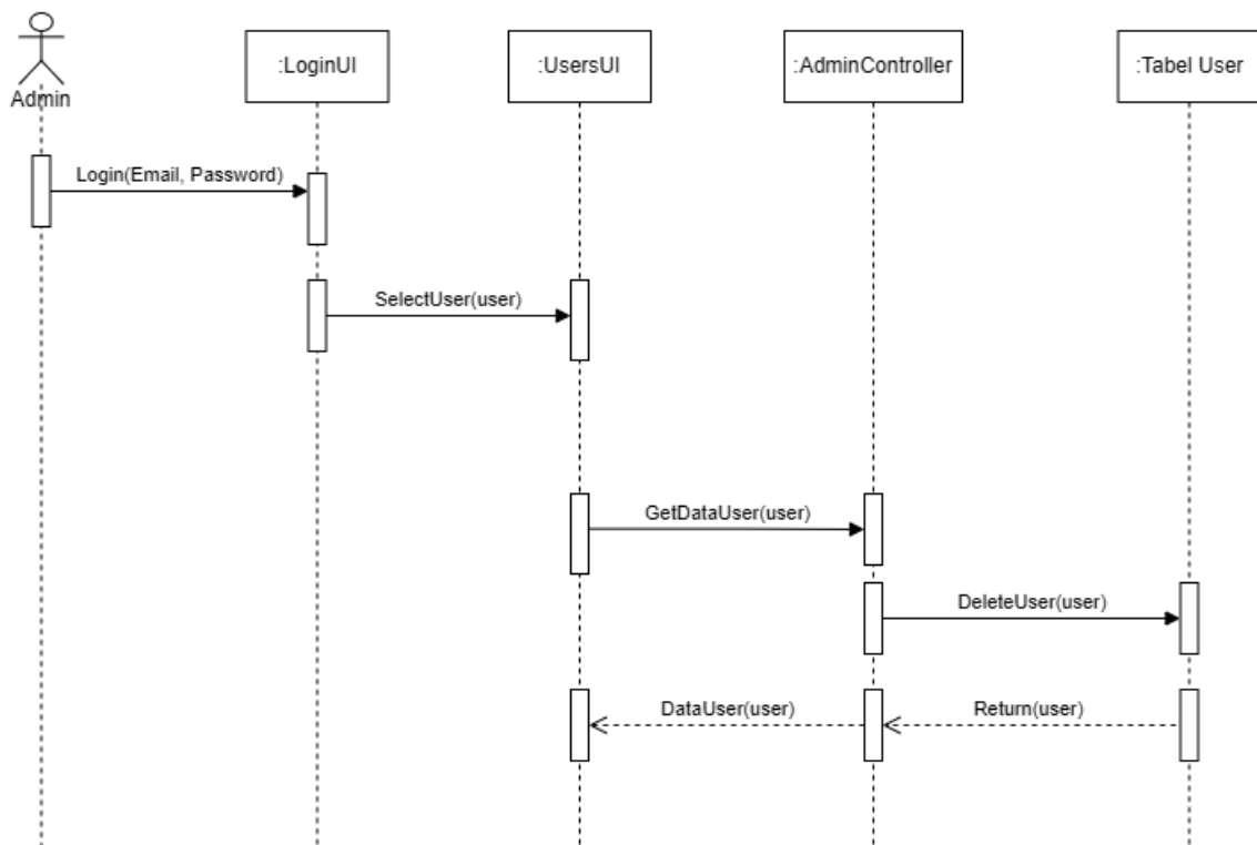
Gambar 3. 12 Sequence Diagram Delete User
