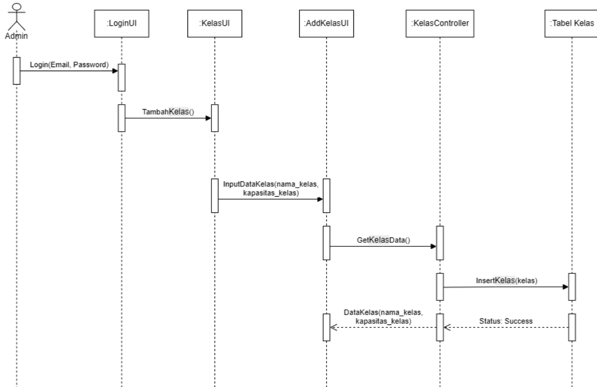
Gambar 3. 29 Sequence Diagram Insert Kelas
