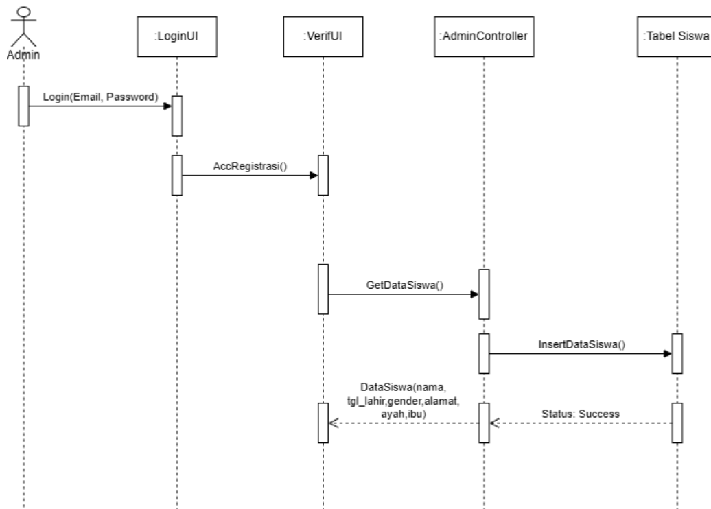
Gambar 3. 15 Sequence Diagram Insert Siswa
