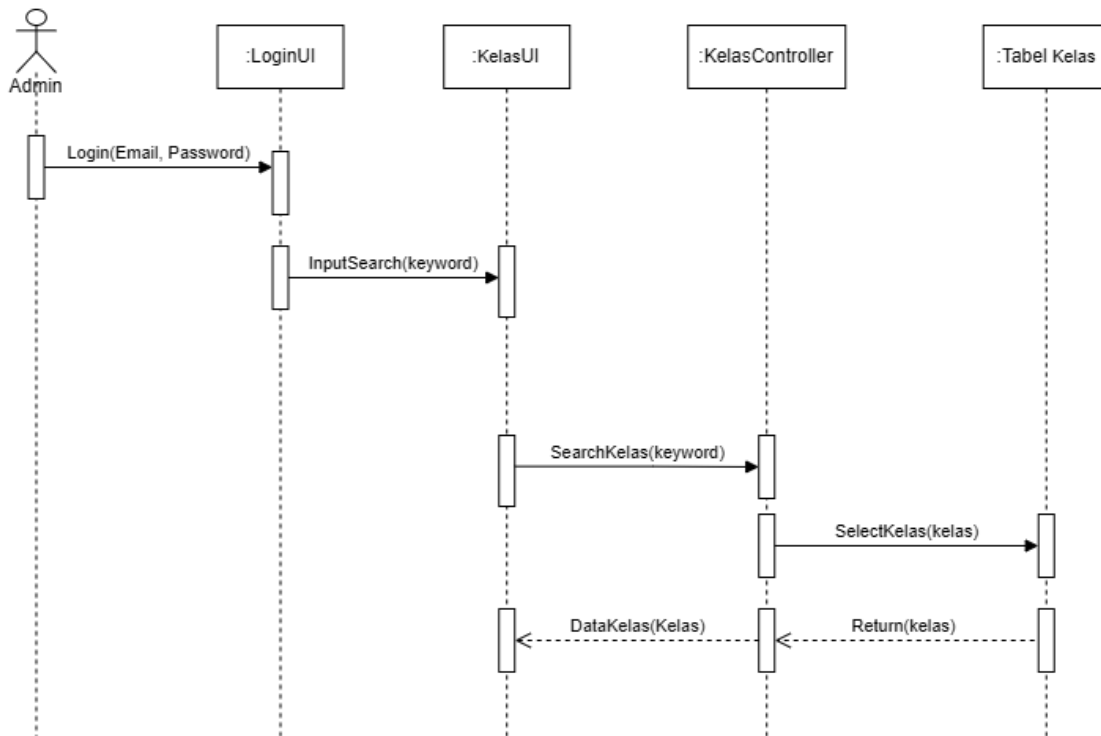
Gambar 3. 32 Sequence Diagram Search Kelas
