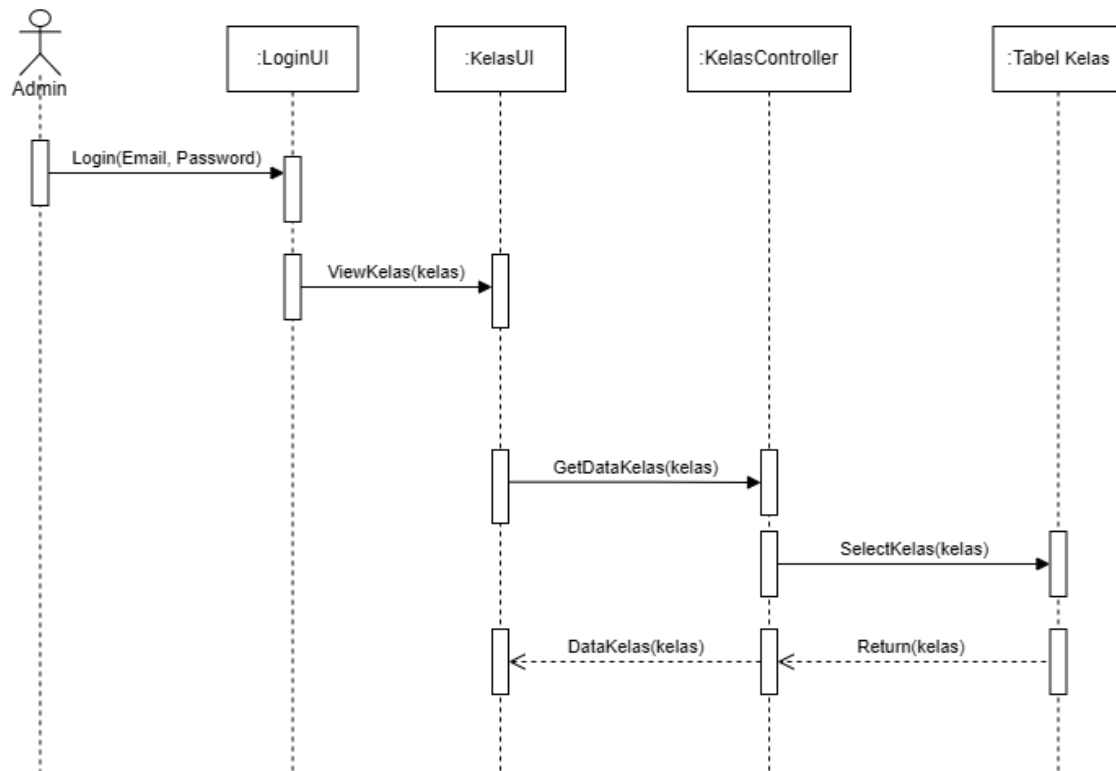
Gambar 3. 33 Sequence Diagram View Kelas
