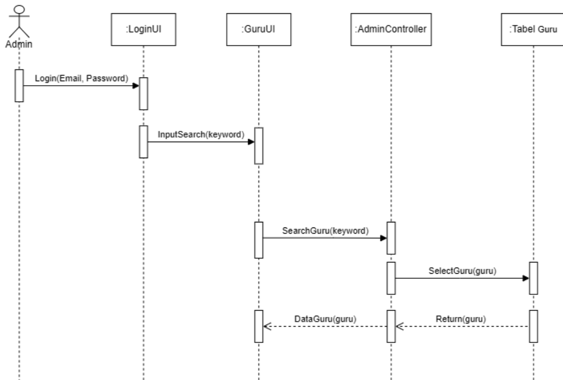
Gambar 3. 27 Sequence Diagram Search Guru
