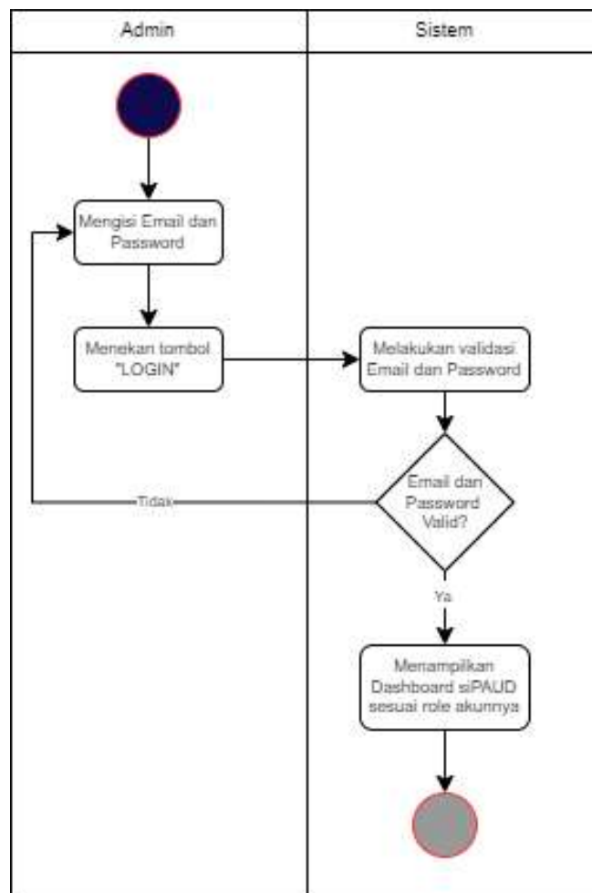
Gambar 3. 3 Activity Diagram Login
