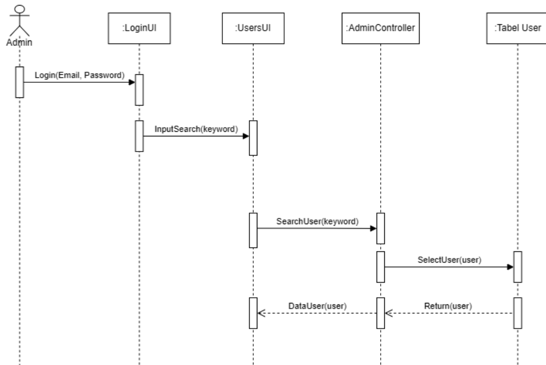
Gambar 3. 13 Sequence Diagram Search User
