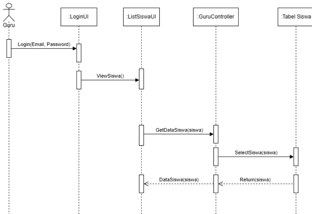
Gambar 3. 36 Sequence Diagram Guru View Siswa
