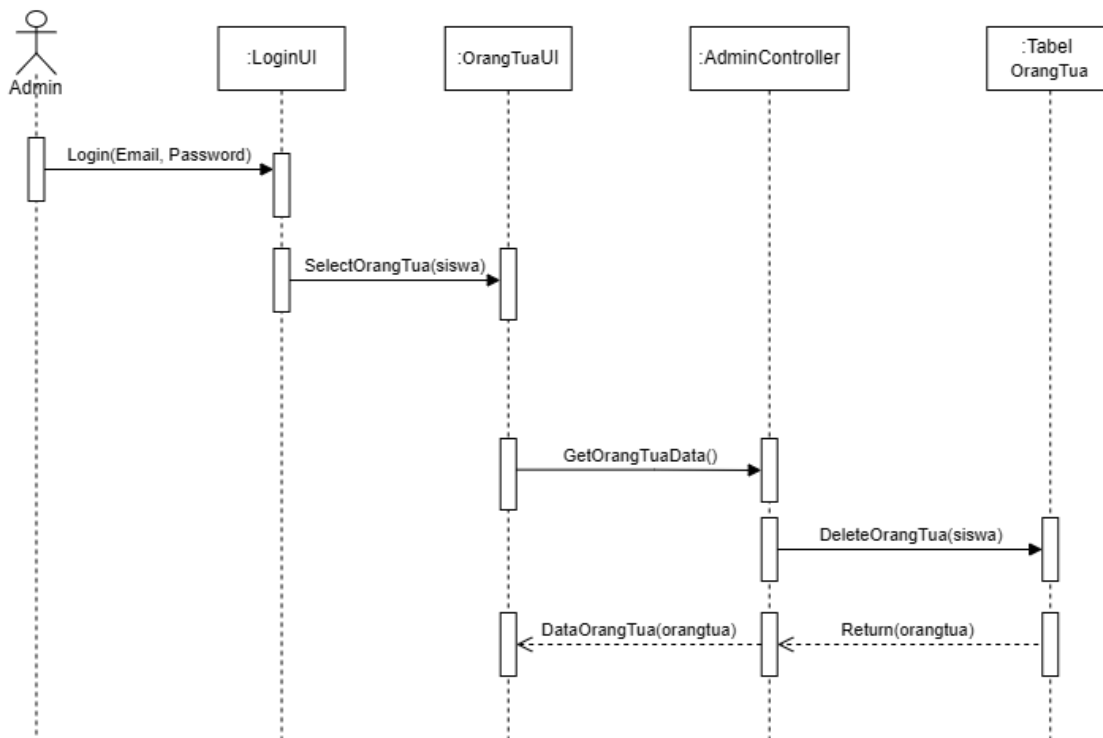
Gambar 3. 22 Sequence Diagram Delete Orang Tua
