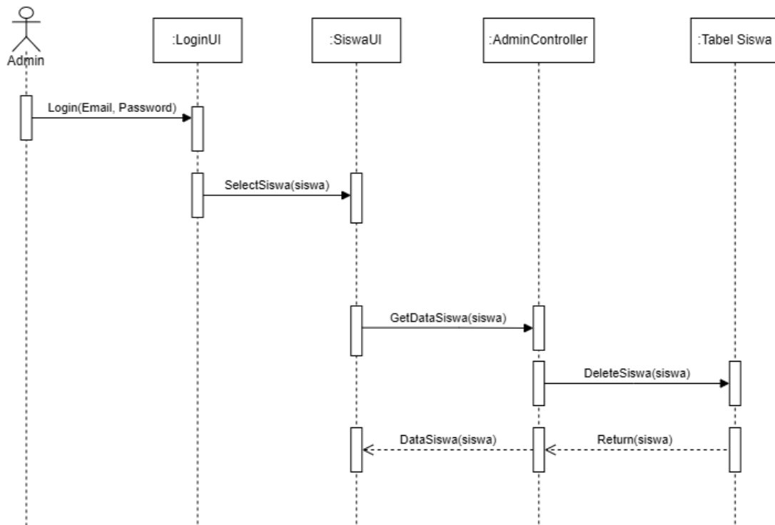
Gambar 3. 17 Sequence Diagram Delete Siswa
