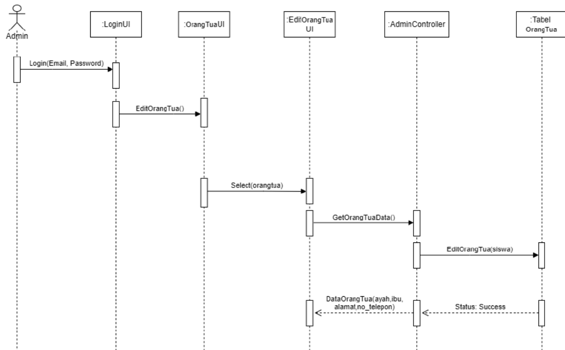
Gambar 3. 21 Sequence Diagram Edit Orang Tua
