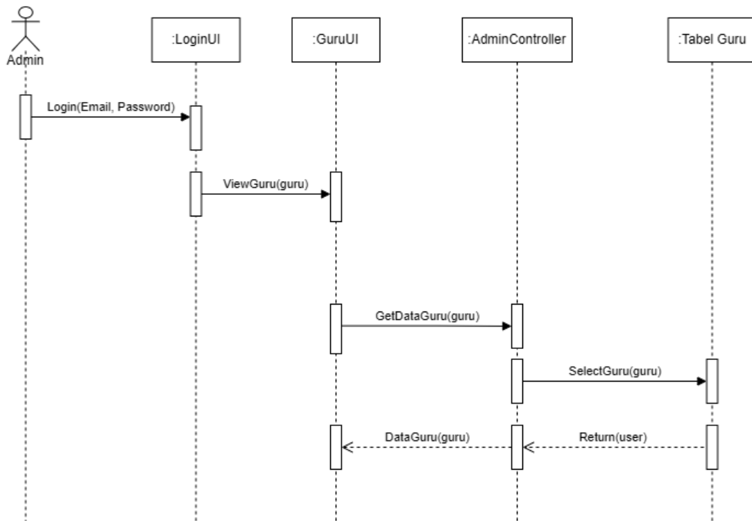
Gambar 3. 28 Sequence Diagram View Guru
