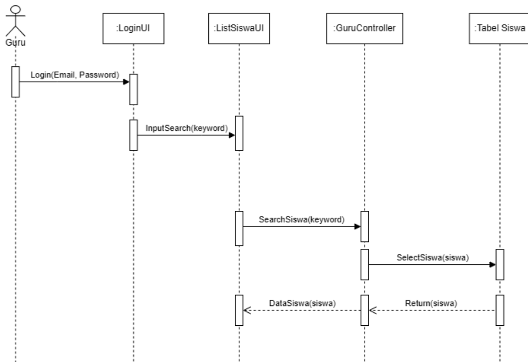
Gambar 3. 35 Sequence Diagram Guru Search Siswa
