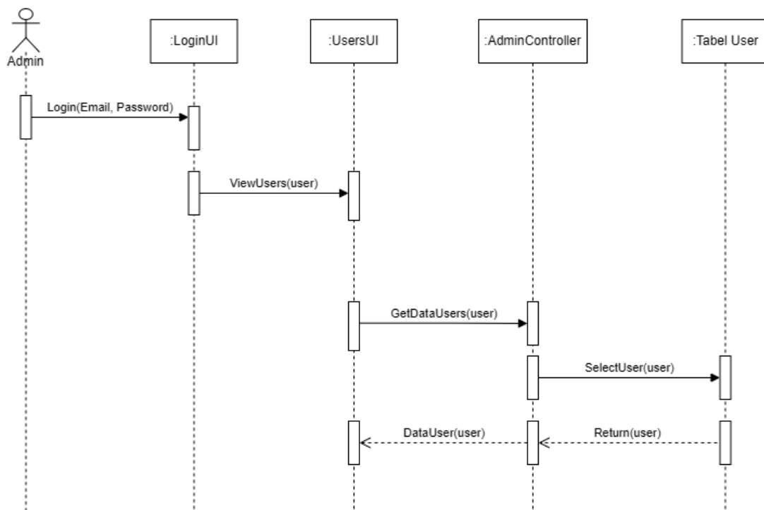
Gambar 3. 14 Sequence Diagram View User
