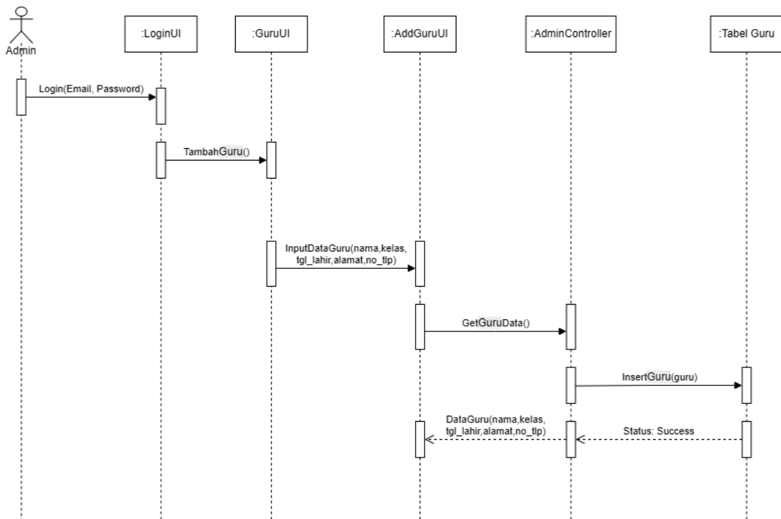
Gambar 3. 24 Sequence Diagram Insert Guru
