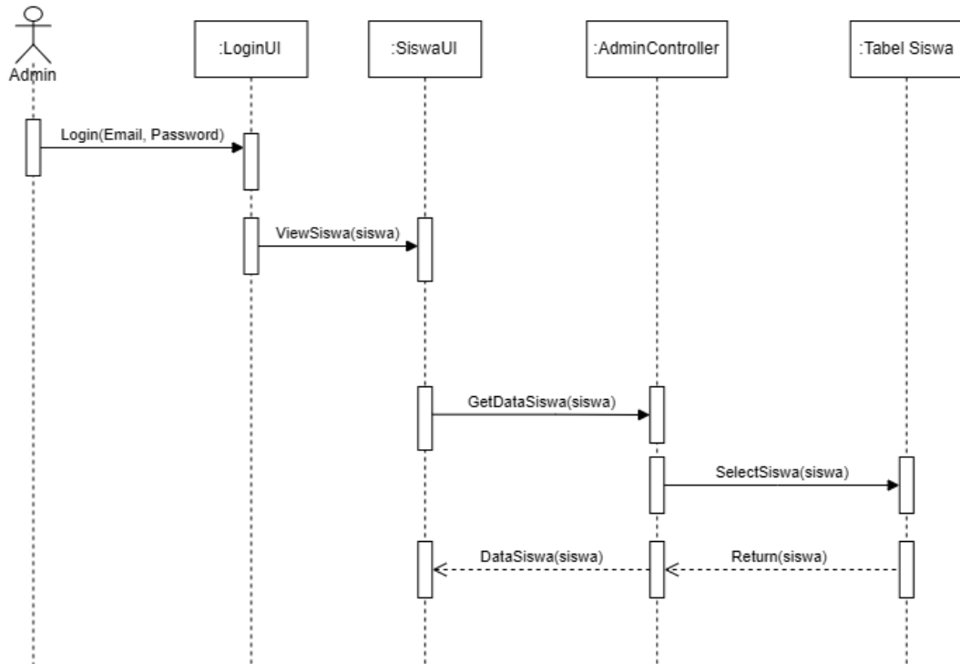
Gambar 3. 19 Sequence Diagram View Siswa
