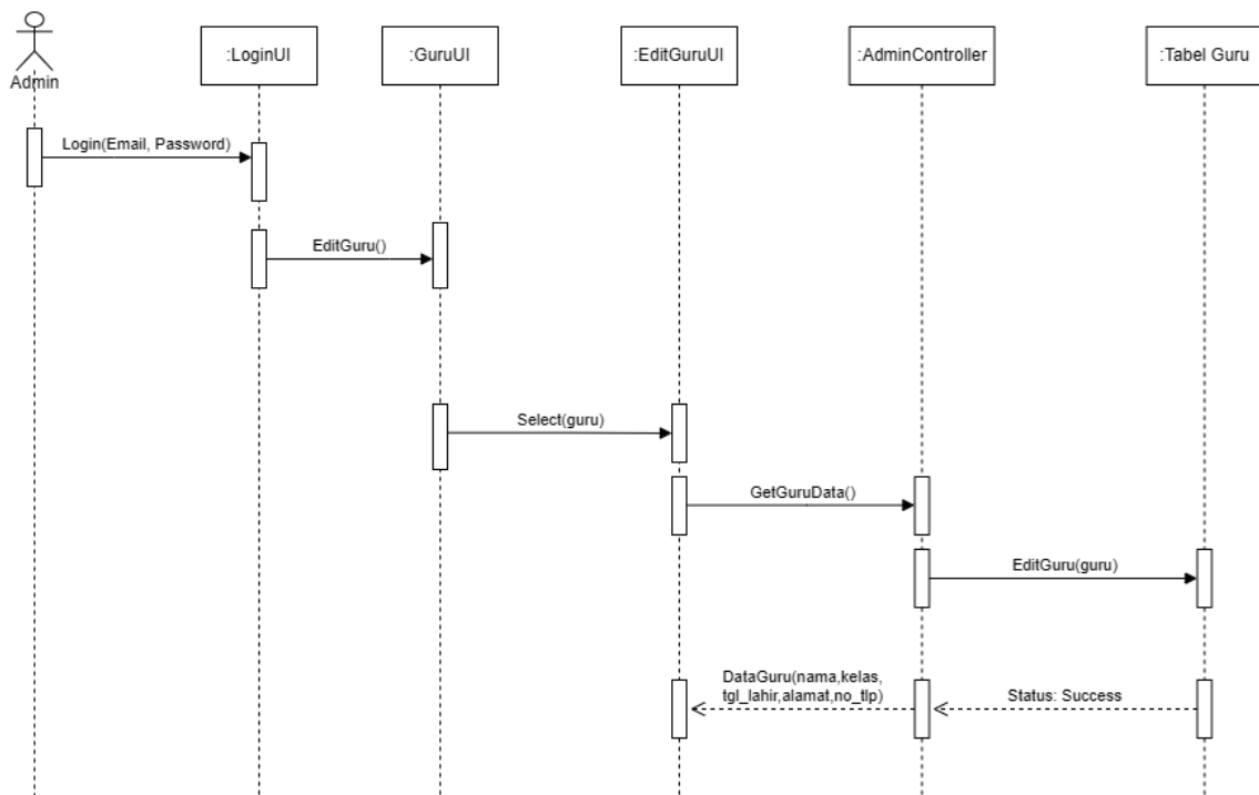
Gambar 3. 25 Sequence Diagram Edit Guru
