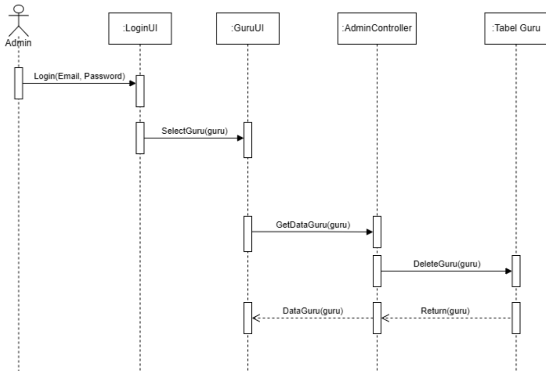
Gambar 3. 26 Sequence Diagram Delete Guru
