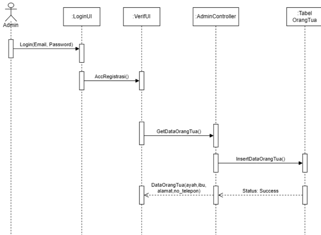
Gambar 3. 20 Sequence Diagram Insert Orang Tua
