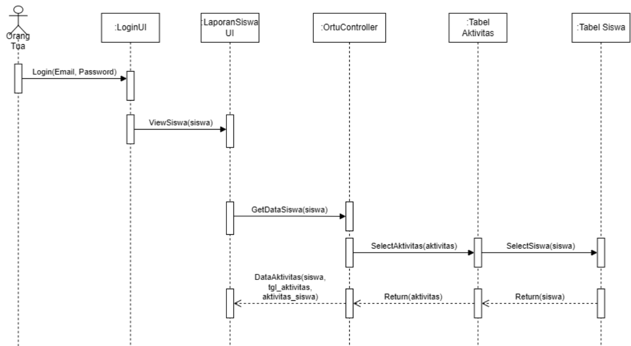
Gambar 3. 37 Sequence Diagram Orang Tua View Siswa
