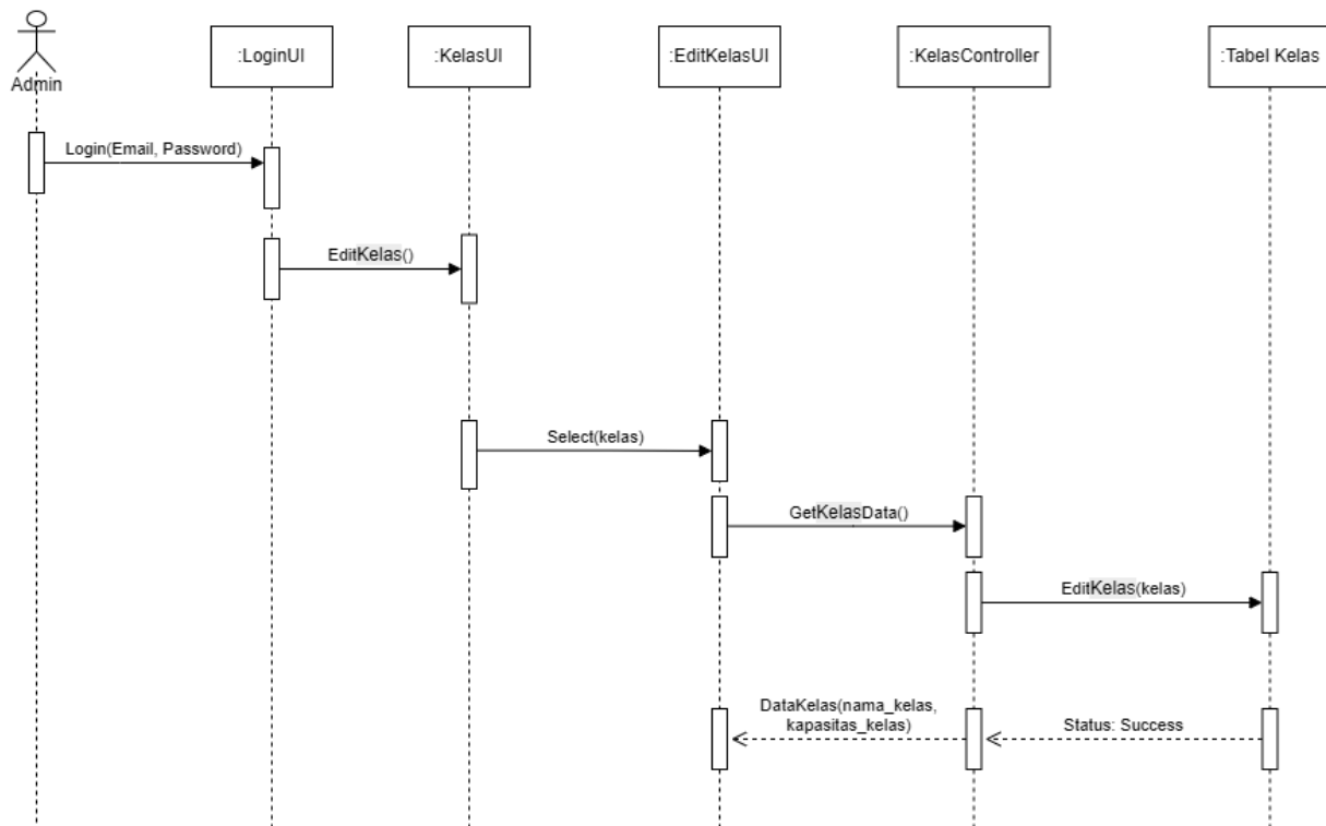
Gambar 3. 30 Sequence Diagram Edit Kelas
